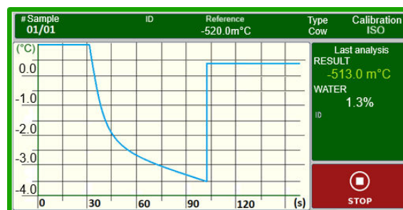
Real-time graph of the cryoscopic point measurement
